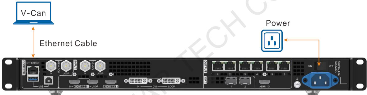
Figure 6-1 Hardware connection
