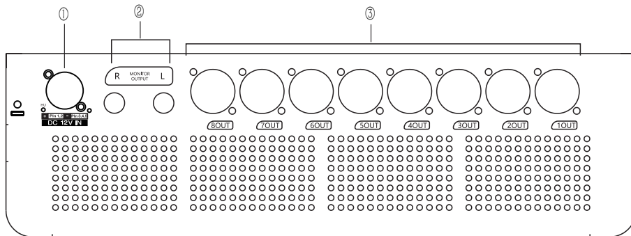
(DG20F Mixer rear panel)
