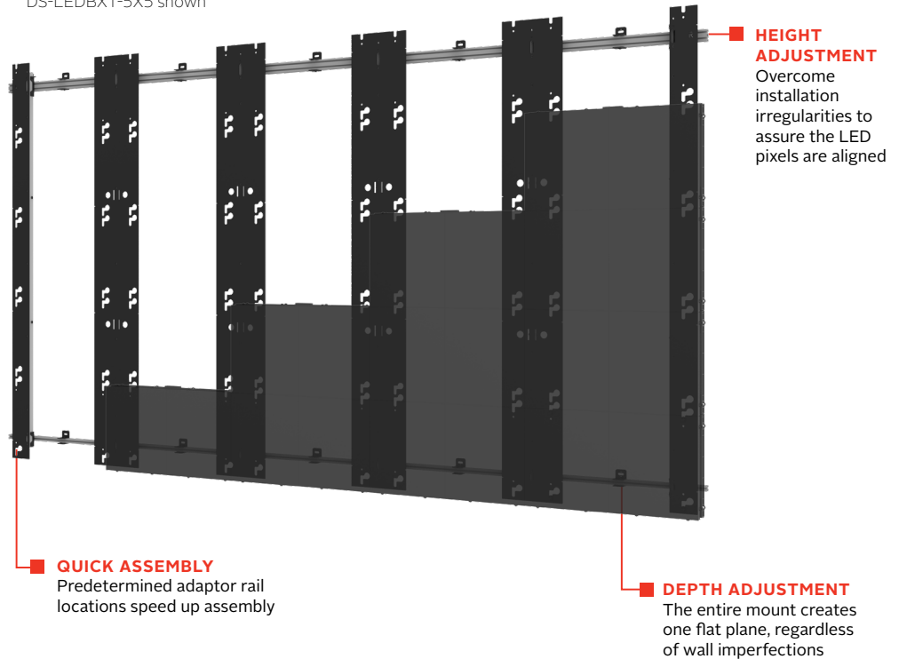
DS-LEDBXT-5X5 shown
